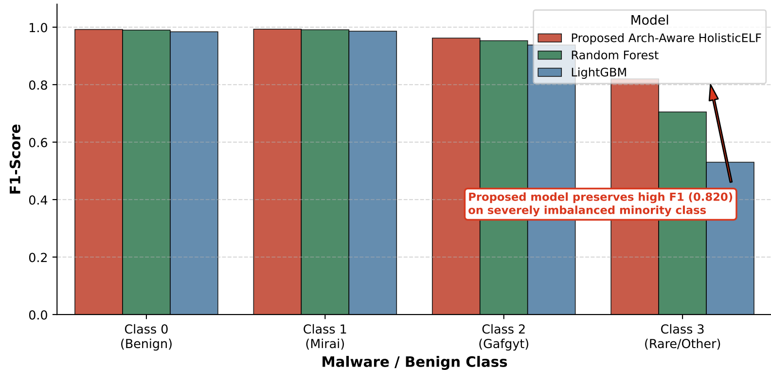
Per-Class F1-Score Breakdown across Malware Families
